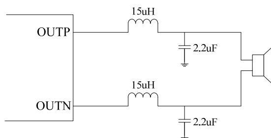
Figure14. Typical LC Output Filter, Cutoff Frequency of 27 kHz, Speaker Impedance = 4 \Omega
