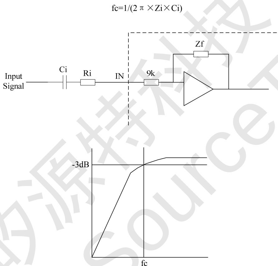
Figure11.highpass filter
